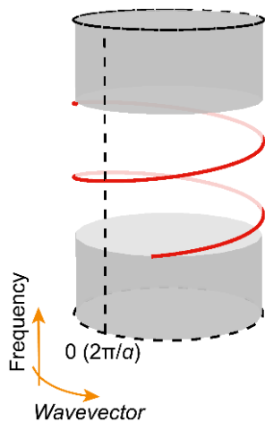
Diagram showing light winding around a Brillouin zone. Credit: NTU.
